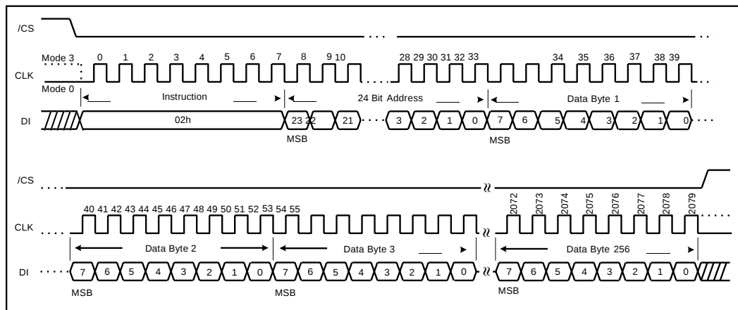
Figure 18a. Page Program Instruction (SPI Mode)
