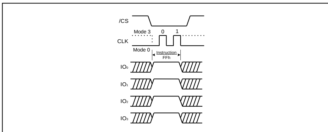
Figure 33. Disable QPI instruction for QPI mode
