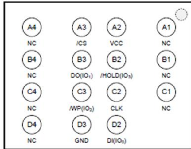
Figure 1C. Pin Assignments,15-Ball WLCSP 0.300mm
